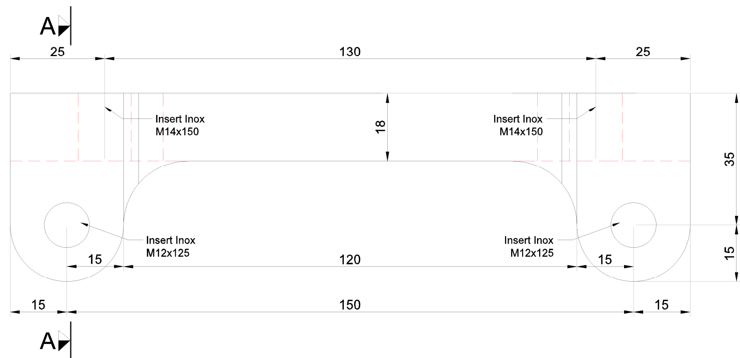
ELEVATION 1 Ech: 1/1
